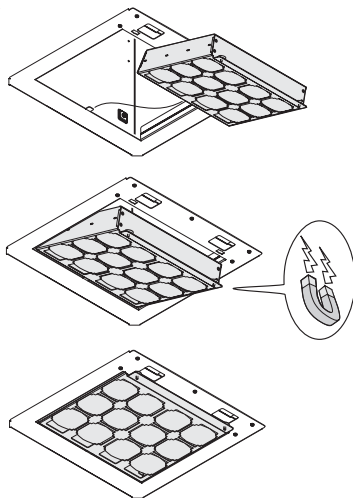
Type SUPCHARC-E
